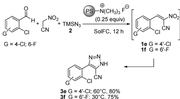
Scheme 1. Amb-F-catalyzed multicomponent one-pot synthesis of 1H-1,2,3-triazoles 3e,f .
